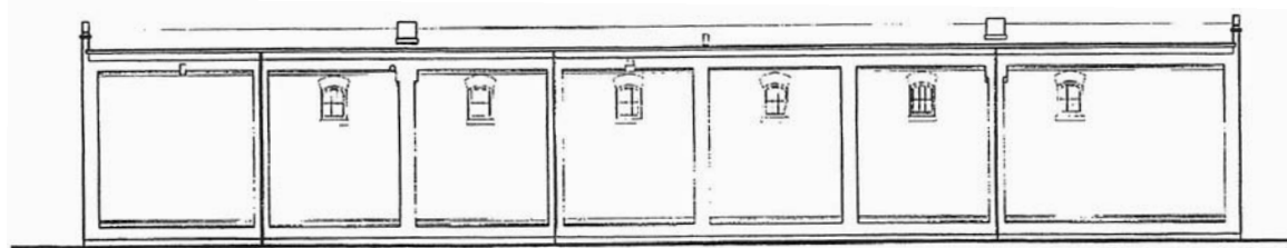
EAST ELEVATION
