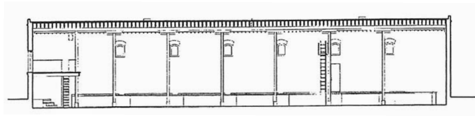
TYPICAL LONGITUDINAL SECTION TANK HOUSE 9
