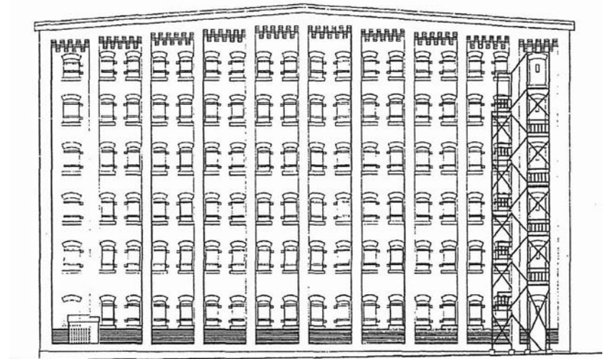
EAST ELEVATION
