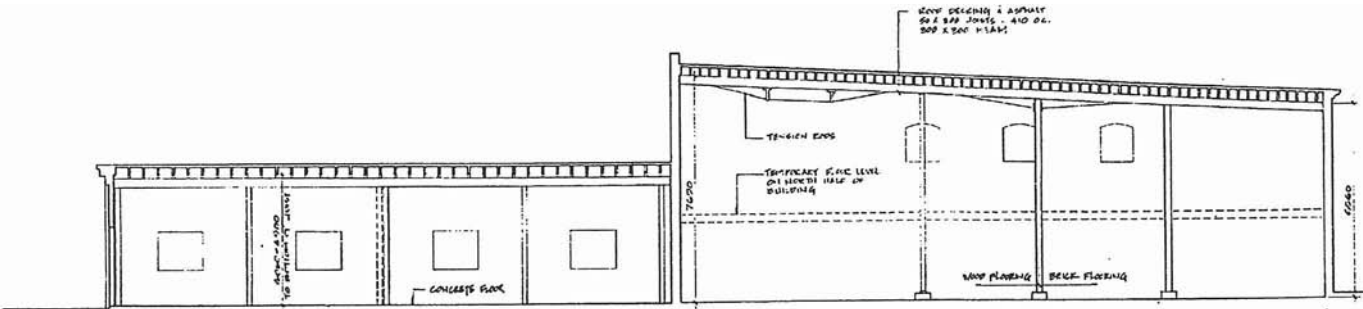
SECTION B-B
