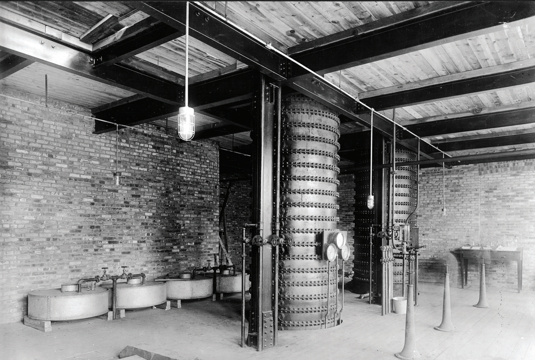
NO 133. MEK · SEC BUTYL & MEK STILLS OPERATING FLOOR NOV 20 1918.
